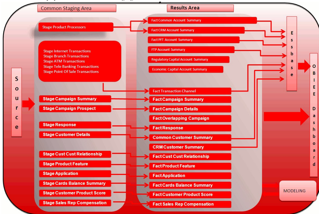
Figure 2. Staging Tables
