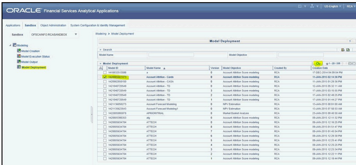
Figure 60. Model Deployment
