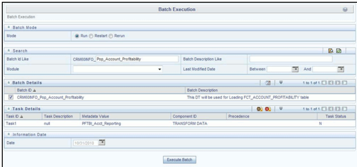
Figure 47. Pop_Account_Profitability
