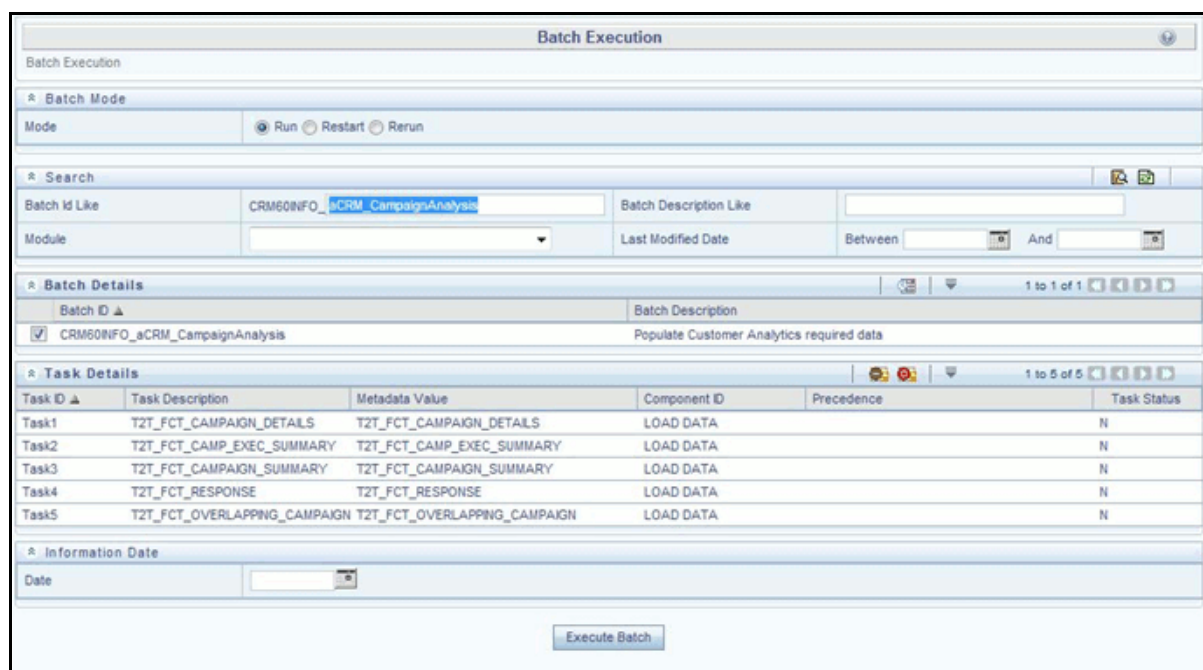
Figure 31. <Infodom>_aCRM_CampaignAnalysis - Task1
